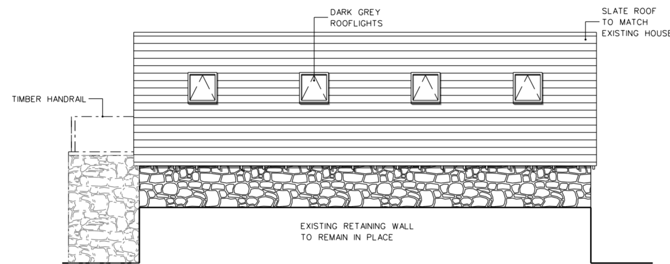
REAR ELEVATION (SOUTH ELEVATION)
