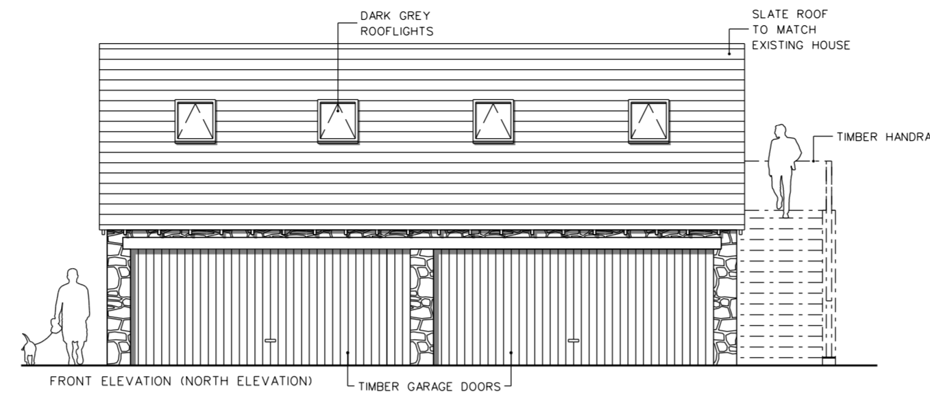
FRONT ELEVATION (NORTH ELEVATION)
